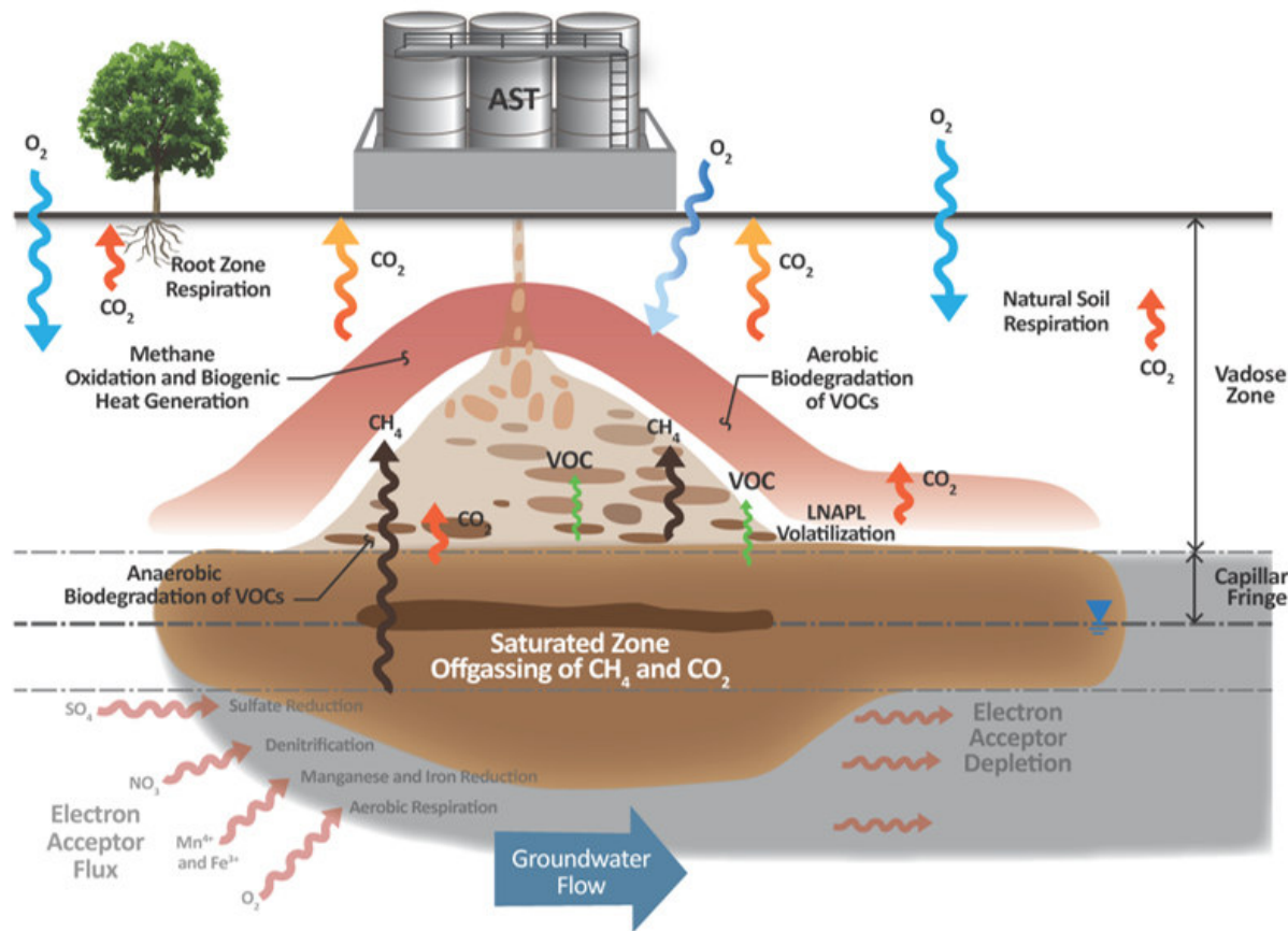
Figure 1. Conceptualization of Vapor Transport-related NSZD Processes at a Petroleum Release Site (with permission from an ongoing American Petroleum Institute NSZD guidance project, pending publication late-2016). CO 2 : Carbon Dioxide. CH 4 : Methane. O 2 : Oxygen. VOC: Volatile Organic Compound. LNAPL: Light Non-Aqueous Phase Liquid; AST: Aboveground Storage Tank.
