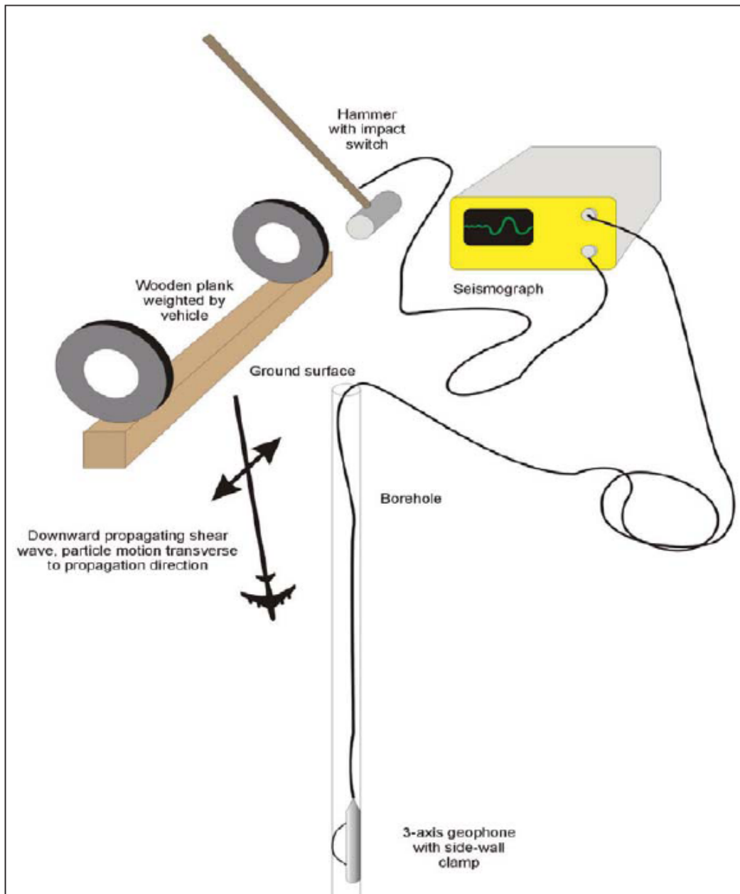
Figure 5. Downhole shear-wave configuration.
