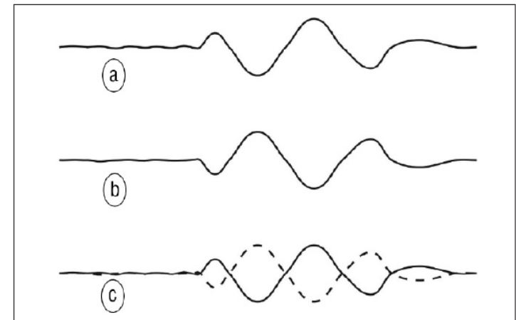
Figure 4. Shear waves reverse polarity when the energy source polarity is reversed.
