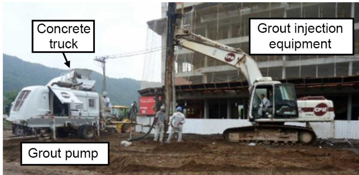
Figure 2. Grouting work in progress at Pontal Oceânico.
